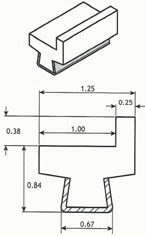
GRA-B/C UHMW/SS
